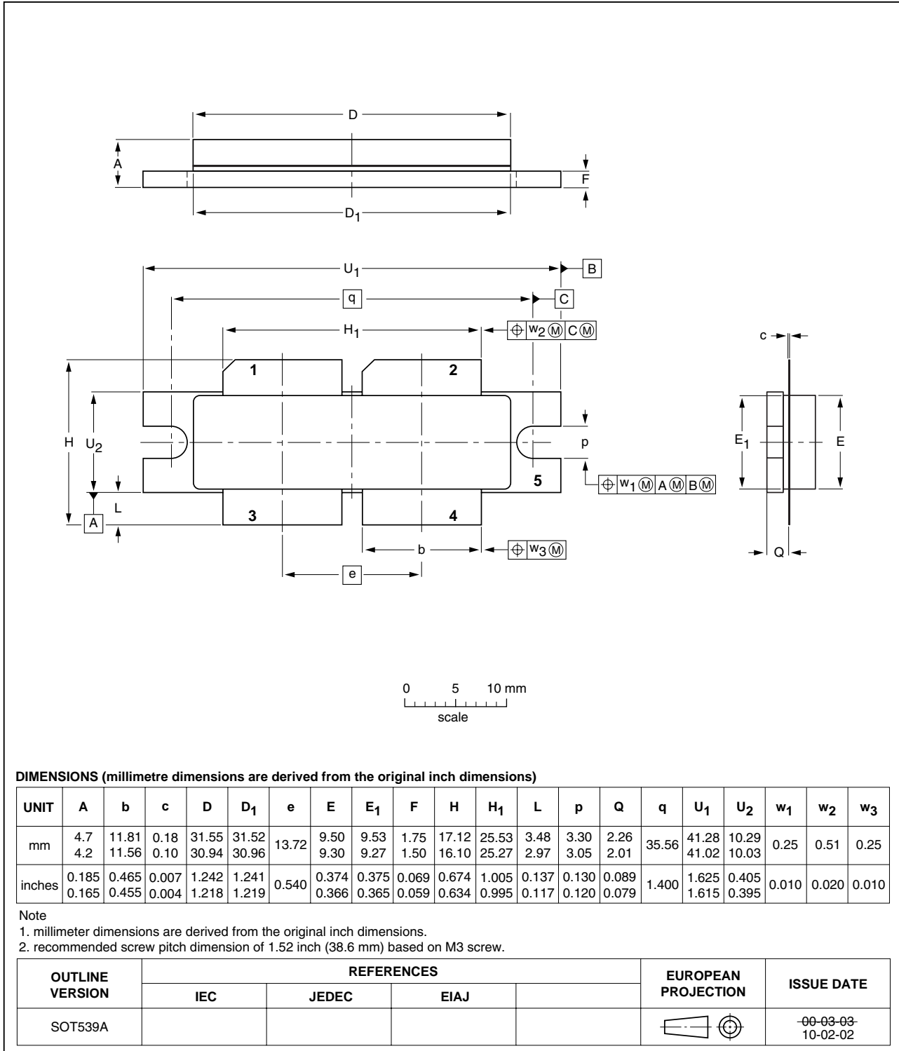
Fig 4. Package outline SOT539A
